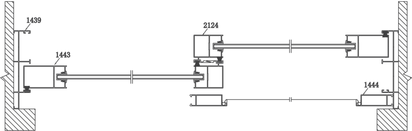
SG (Sliding Horizontal Section Details)
