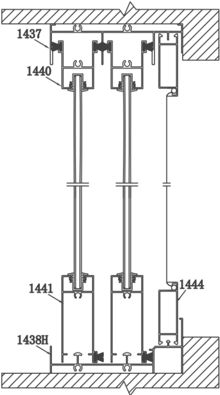
SG (Sliding Vertical Section Details)
